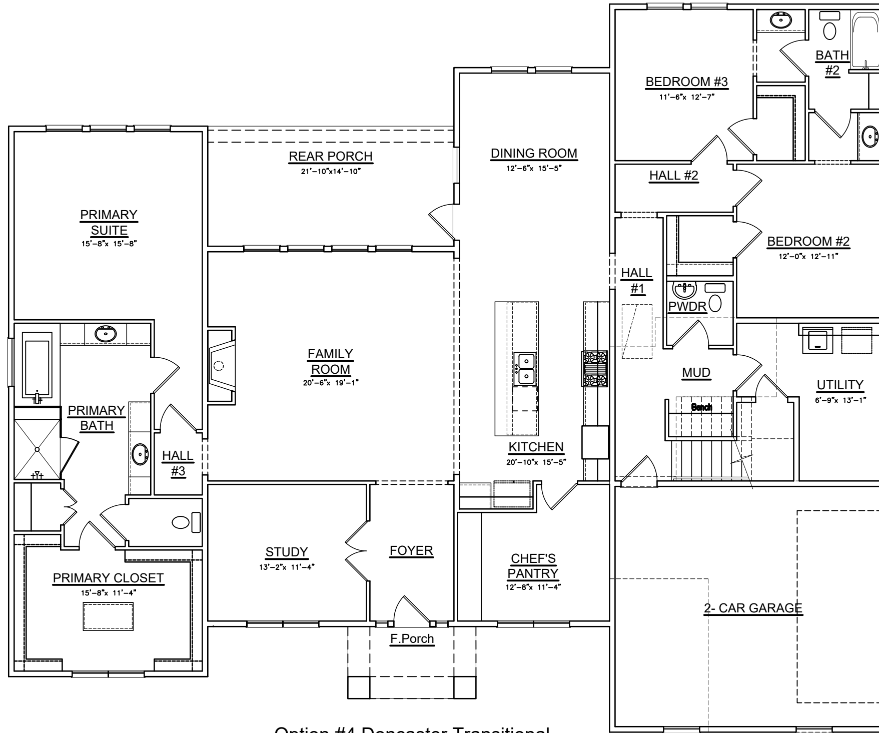
Option #4 Doncaster Transitional w/ 2nd Floor Flex Room & Half Bath
