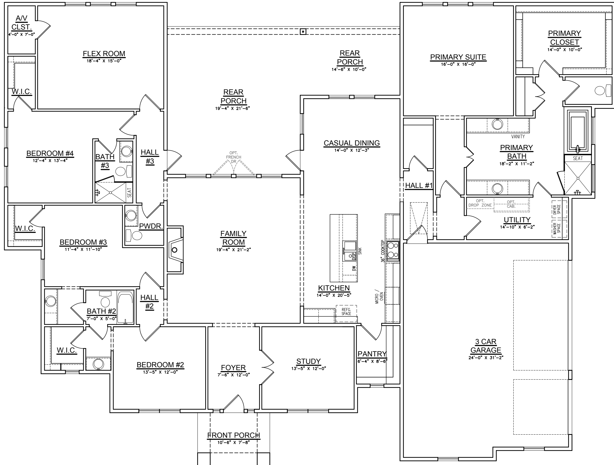
Option #7 Abbott Transitional with 4th Bedroom, Extended R. Porch and 3-Car Garage
