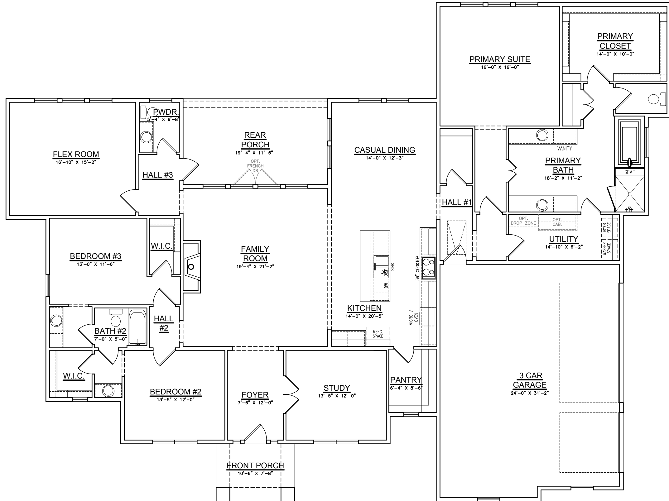
Option #3 Abbott Transitional with Garage Opt. 3-Car Garage
