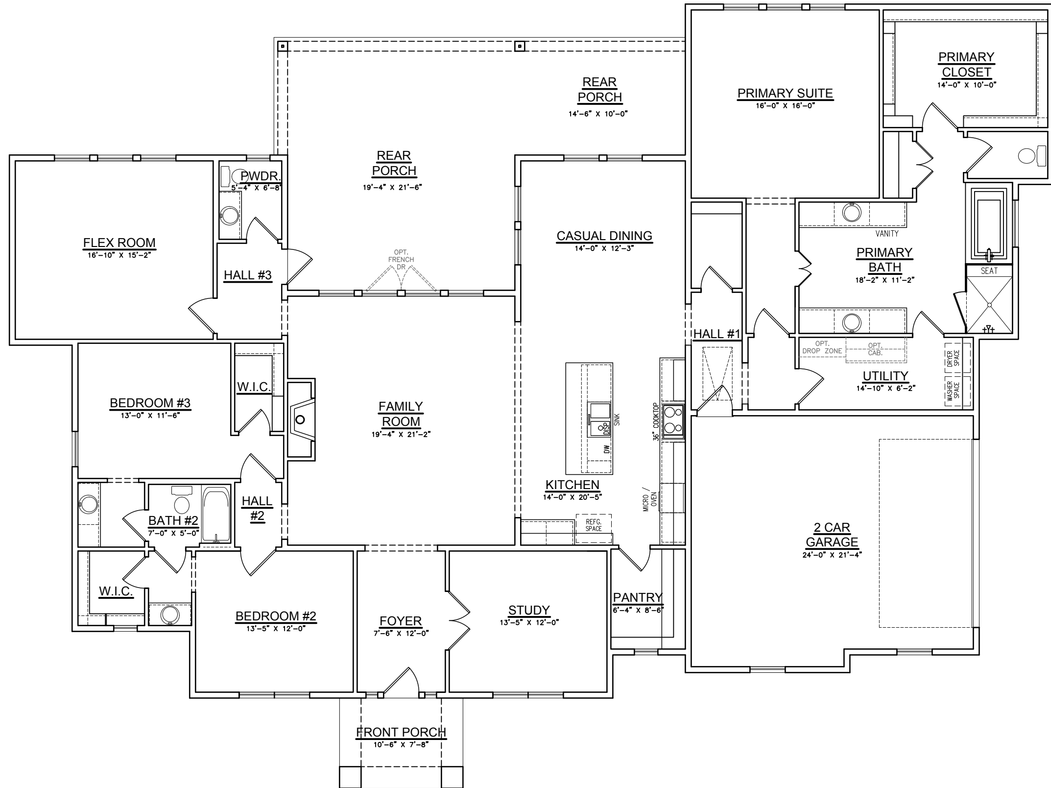
Option #2 Abbott Transitional with Extended R. Porch
