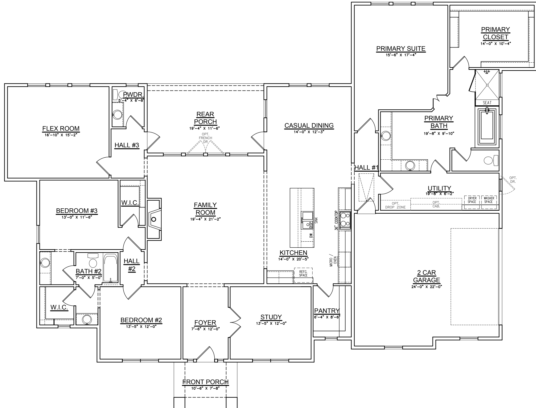
Option #8 Abbott Transitional with Traditional Primary Bath
