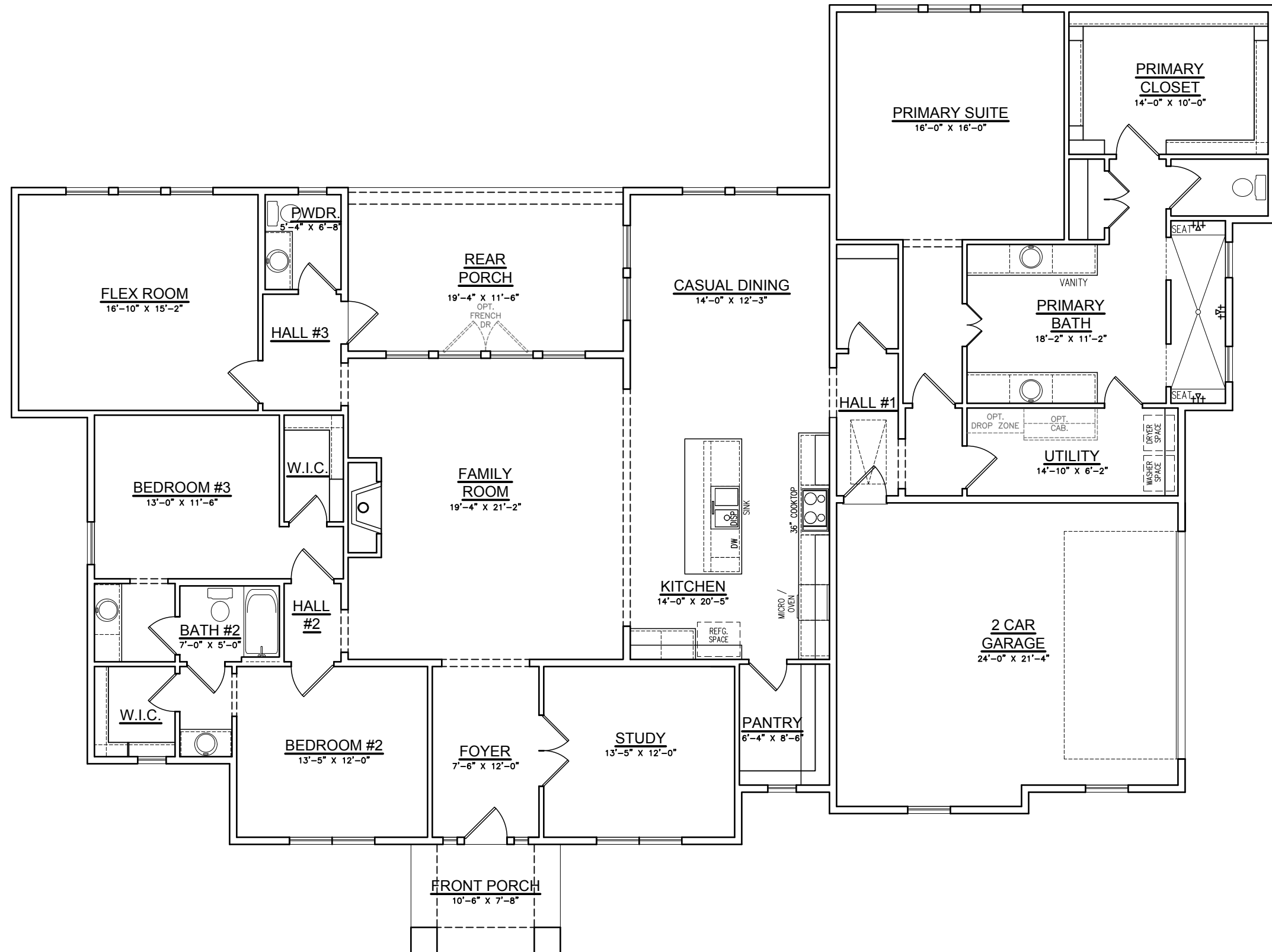
Option #1 Abbott Transitional with Primary Suite Opt. No Primary Bath Tub
