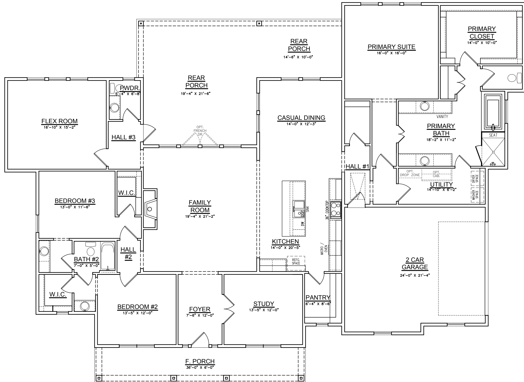
Option #2 Abbott Hill Country with Extended R. Porch
