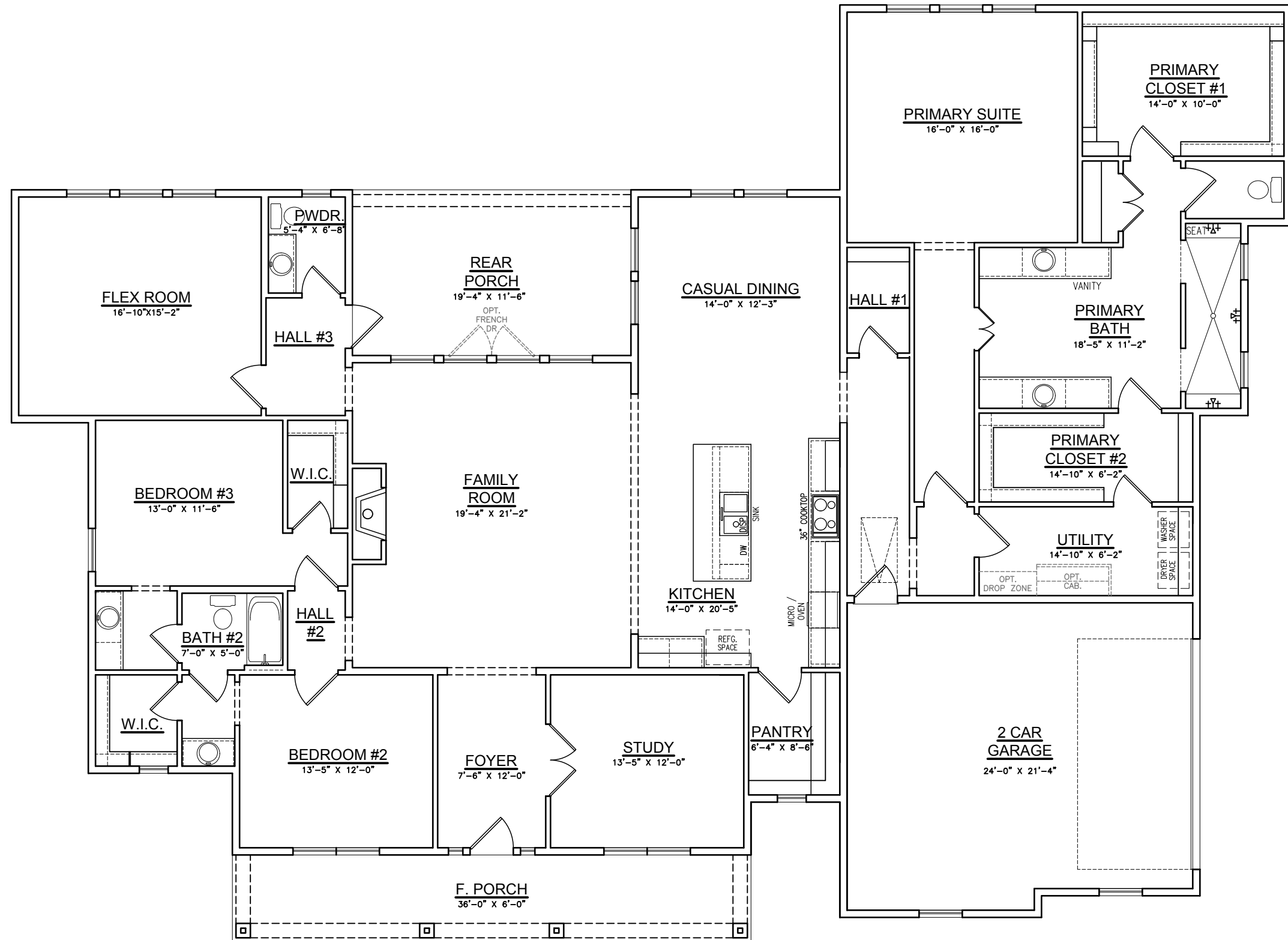
Option #5 Abbott Hill Country with Primary Suite Opt. Two Primary Closets W/ No Primary Bath Tub
