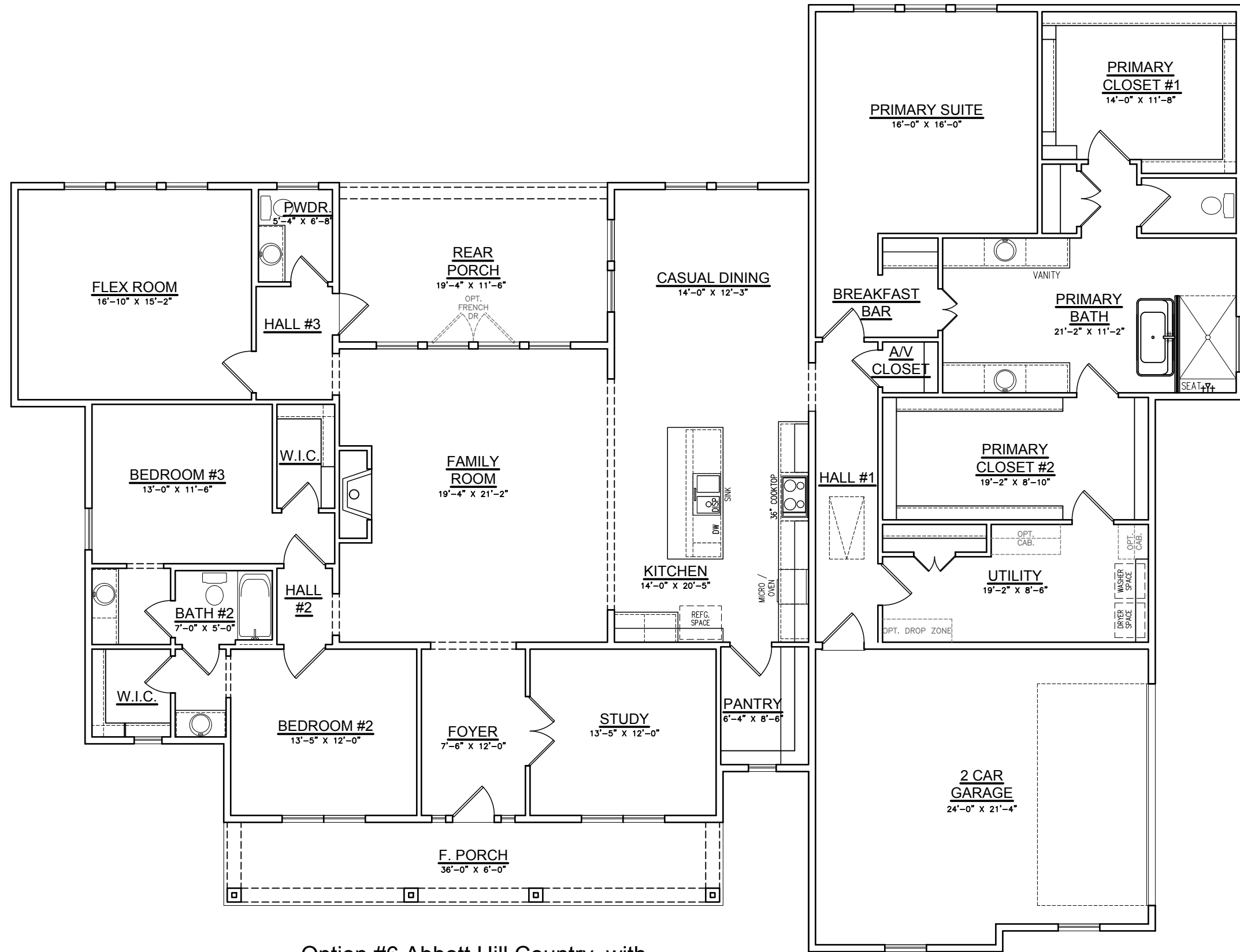
Option #6 Abbott Hill Country with Primary Suite Opt. Larger Primary Suite
