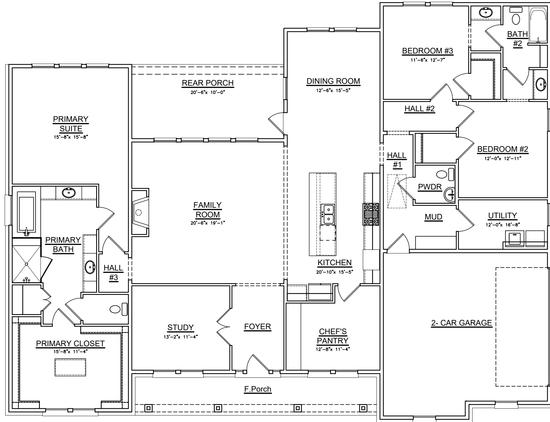
Doncaster Modern Acadian Base Plan
