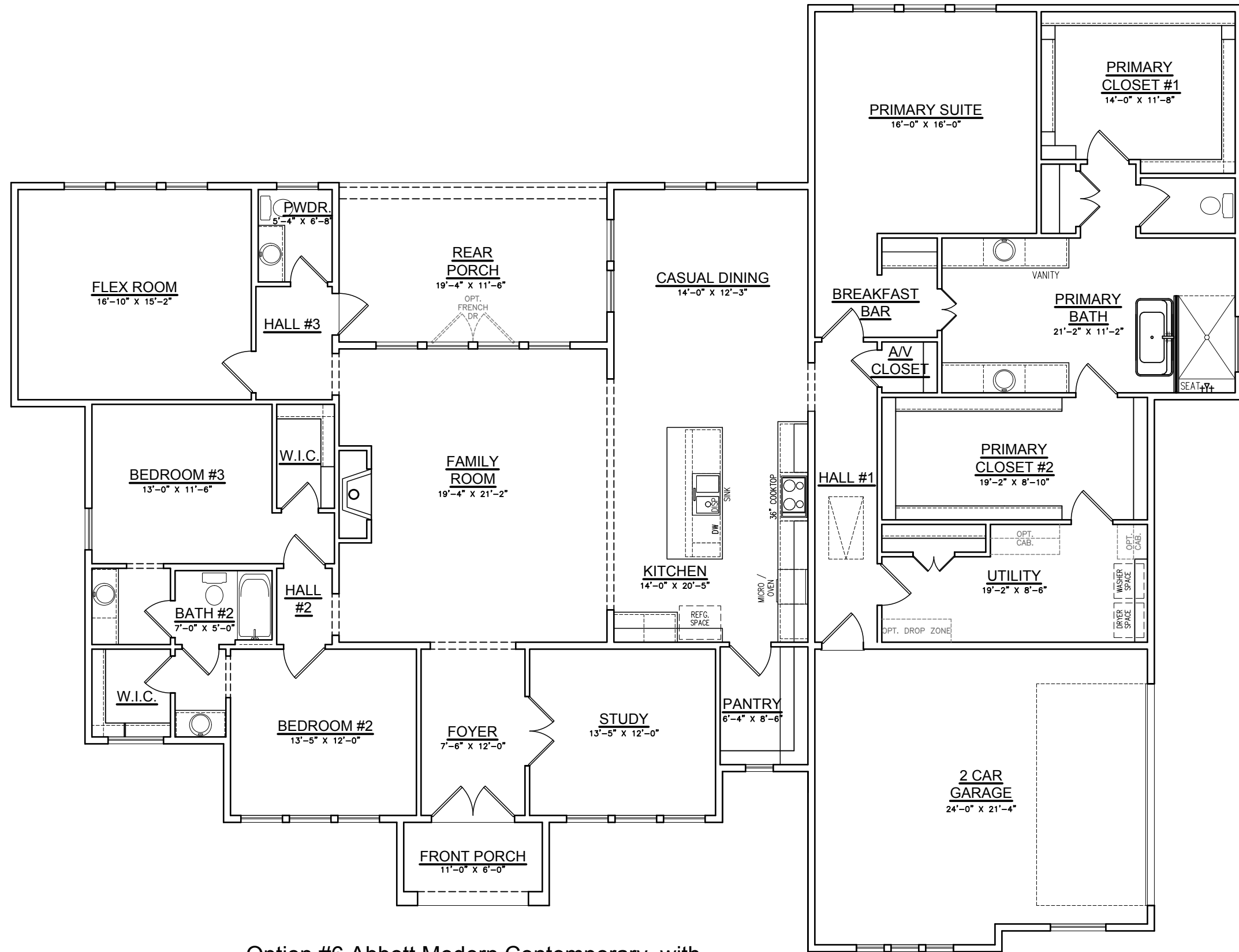
Option #6 Abbott Modern Contemporary with Primary Suite Opt. Larger Primary Suite
