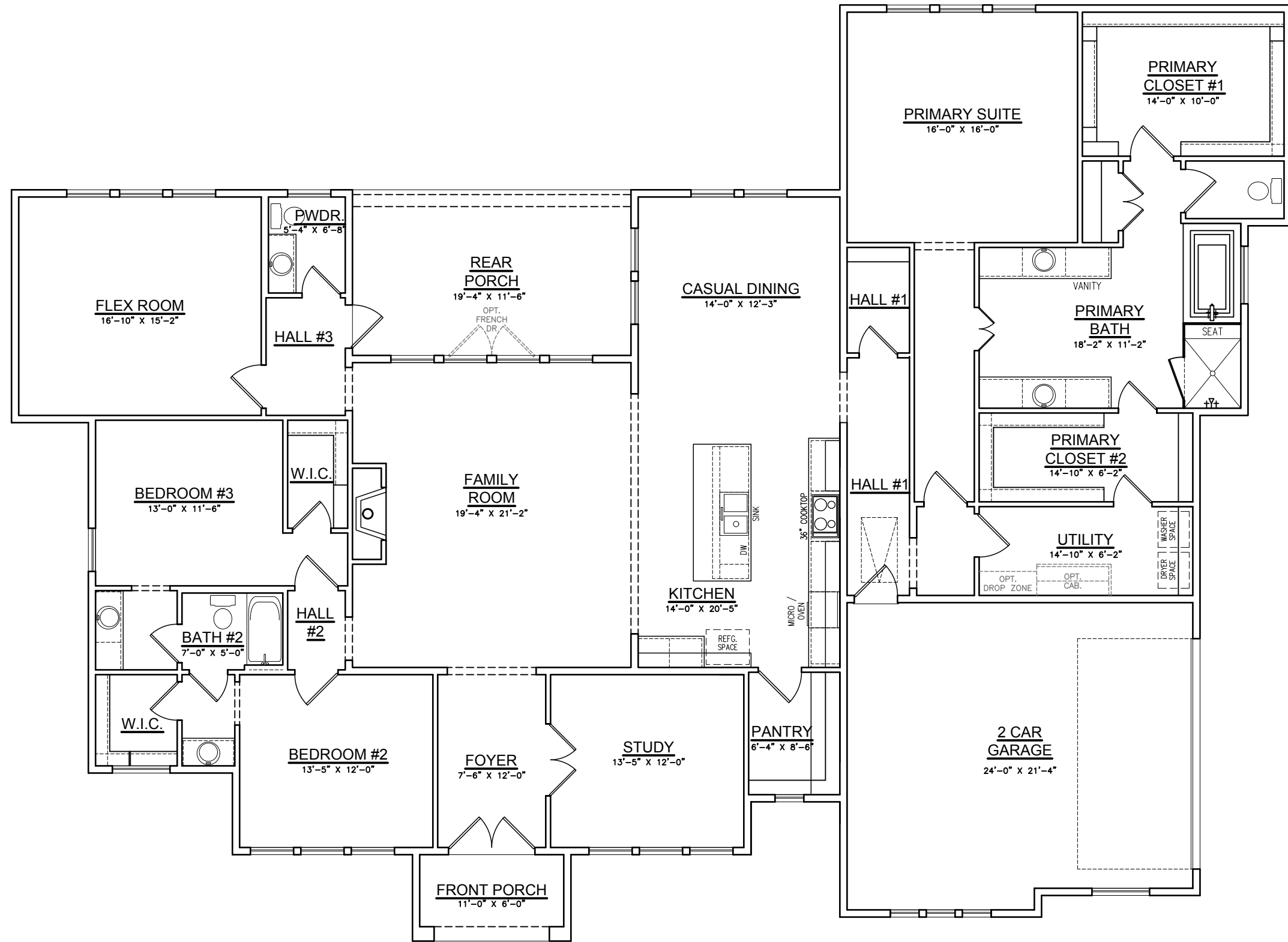
Option #4 Abbott Modern Contemporary with Primary Suite Opt. Two Primary Closets
