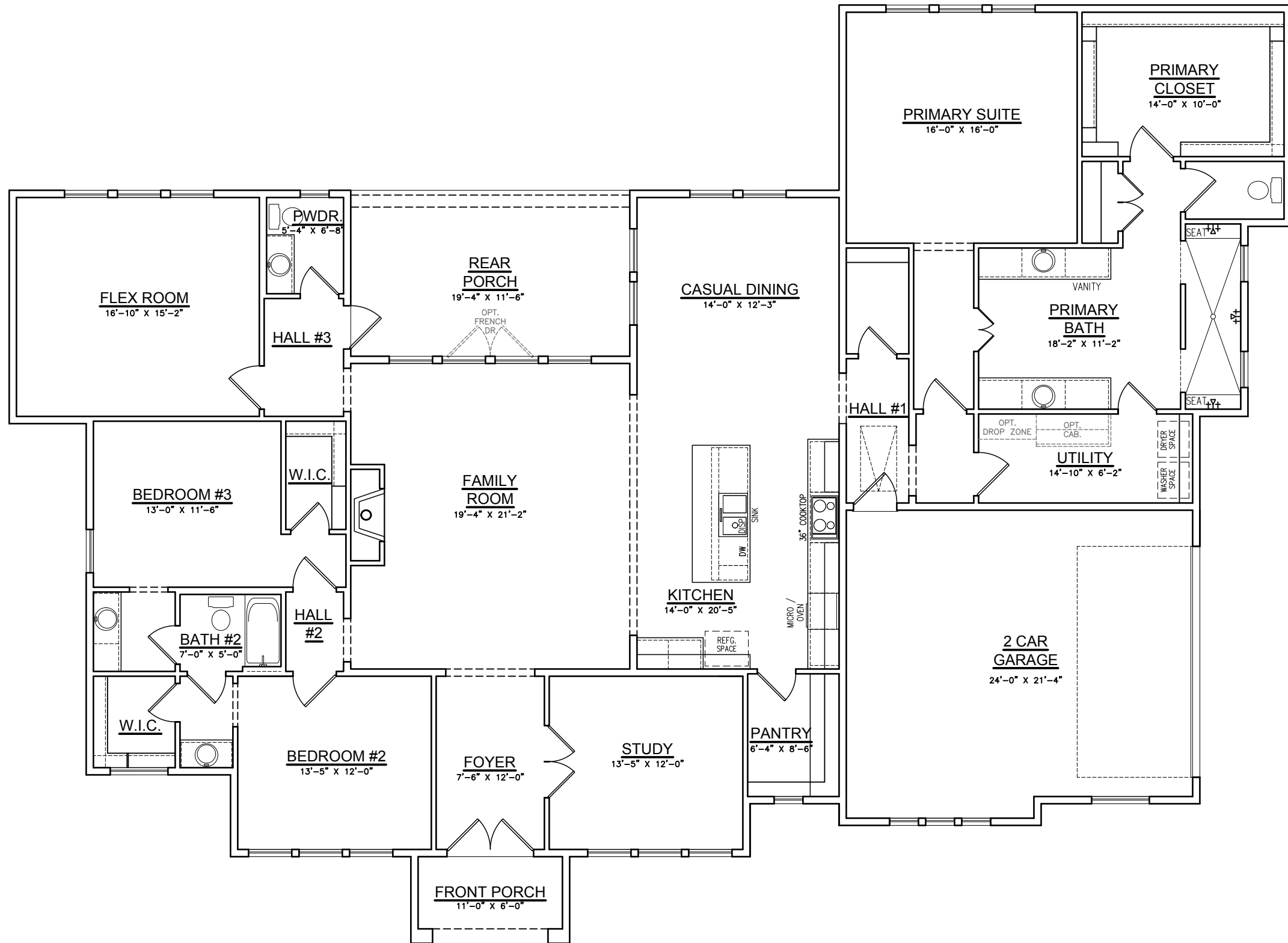
Option #1 Abbott Modern Contemporary with Primary Suite Opt. No Primary Bath Tub
