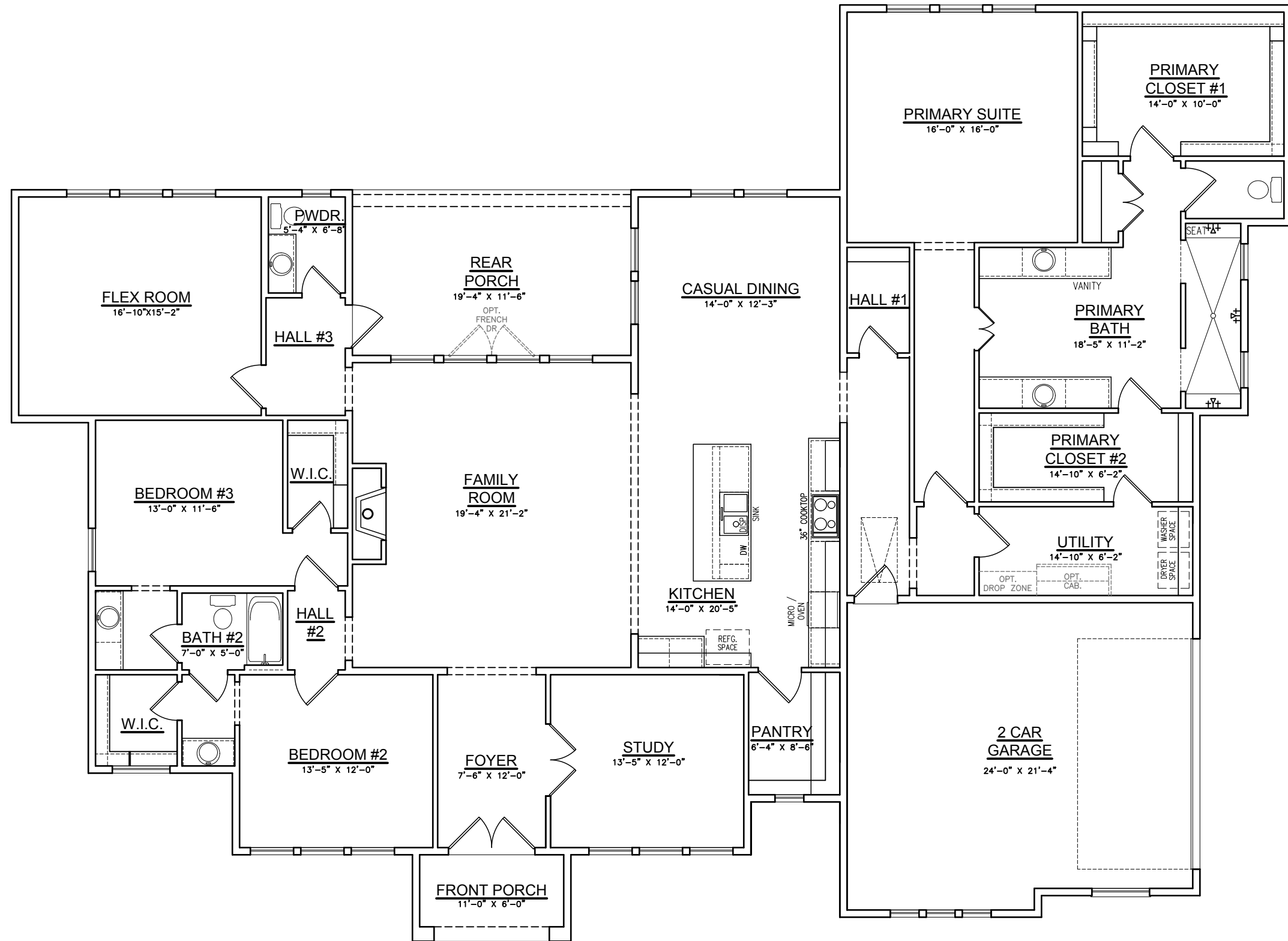
Option #5 Abbott Modern Contemporary with Primary Suite Opt. Two Primary Closets W/ No Primary Bath Tub
