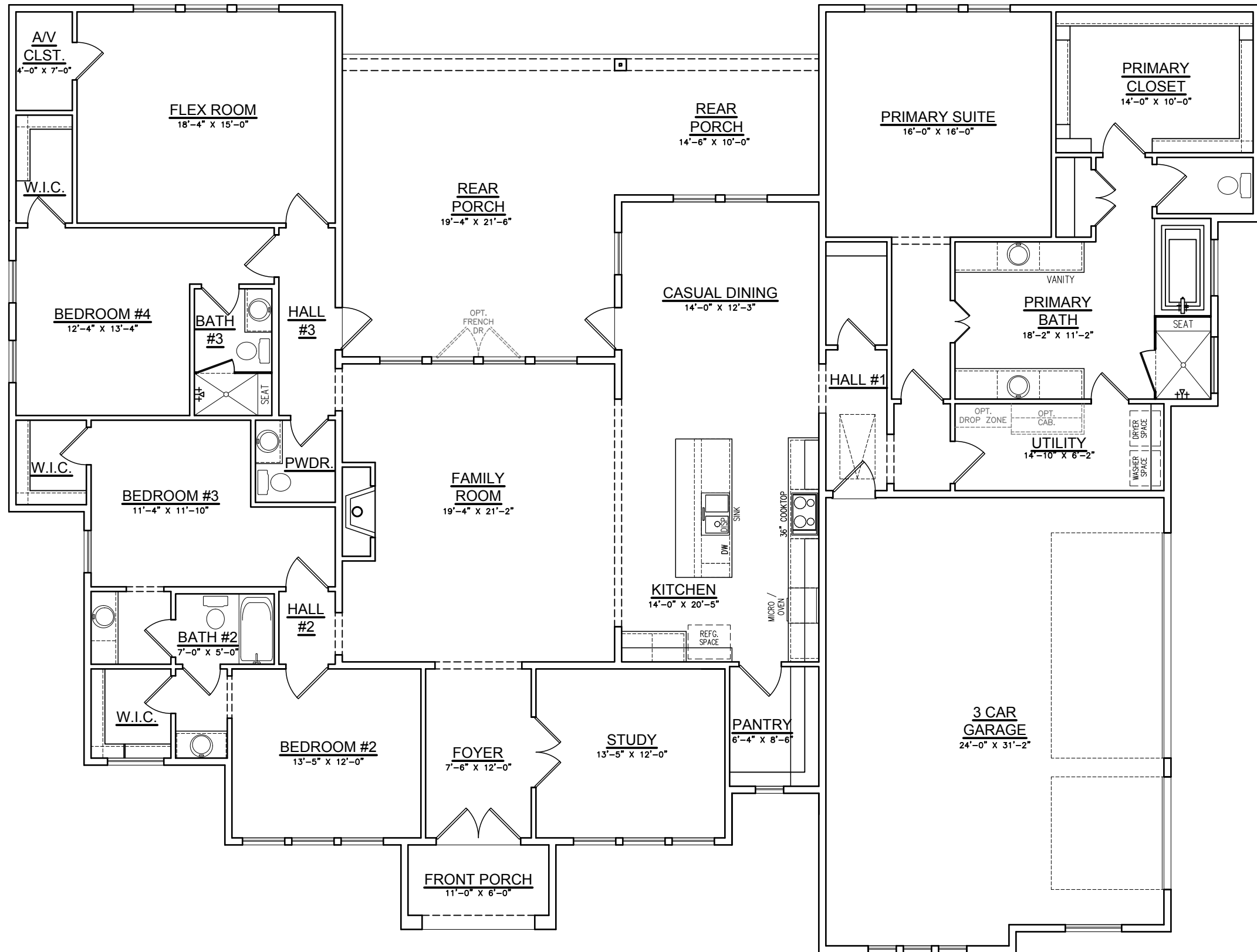
Option #7 Abbott Modern Contemporary with 4th Bedroom, Extended R. Porch and 3-Car Garage
