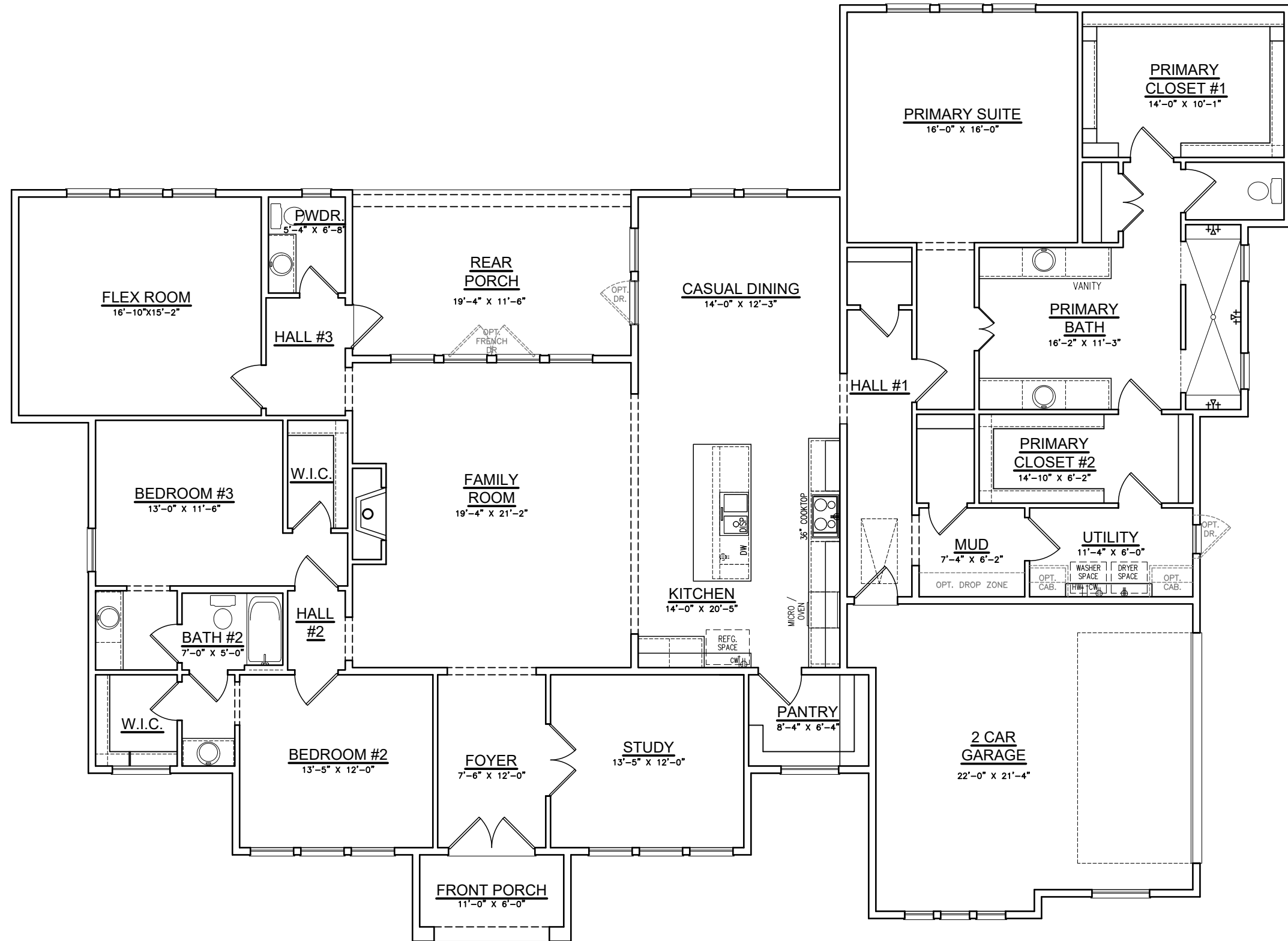
Option #5 Abbott Modern Contemporary w/ Primary Suite Opt. Two Primary Closets w/ No Primary Bath Tub
