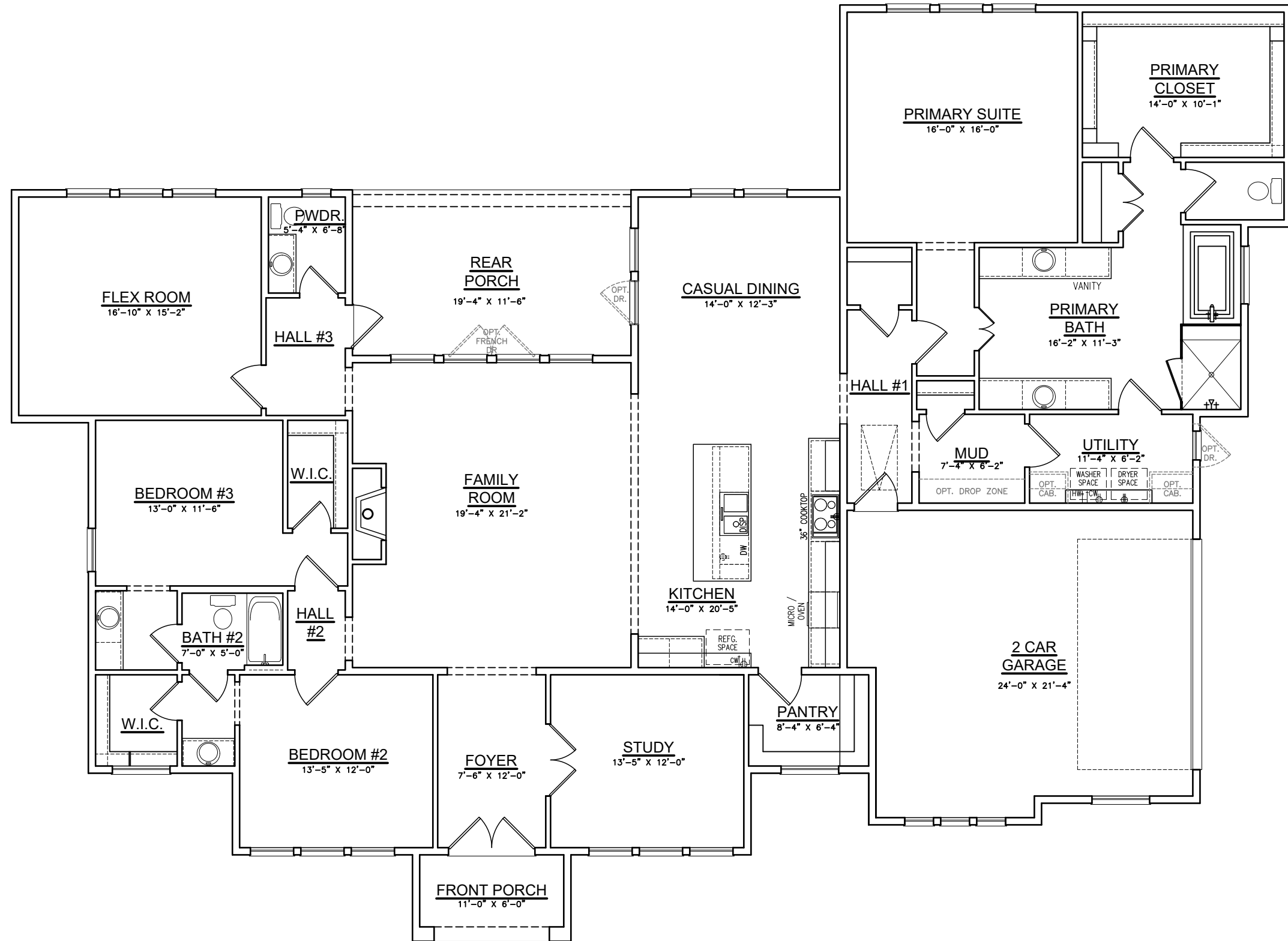
Abbott Modern Contemporary Base Plan
