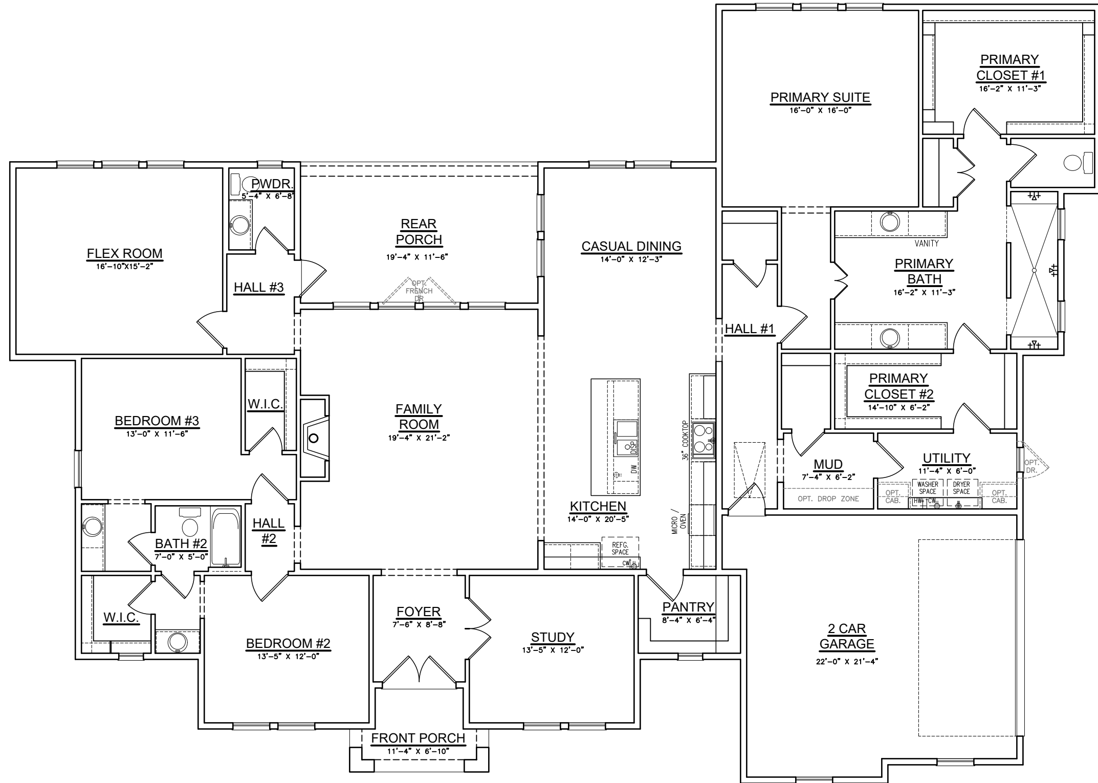
Option #5 Abbott French Revival with Primary Suite Opt. Two Primary Closets W/ No Primary Bath Tub
