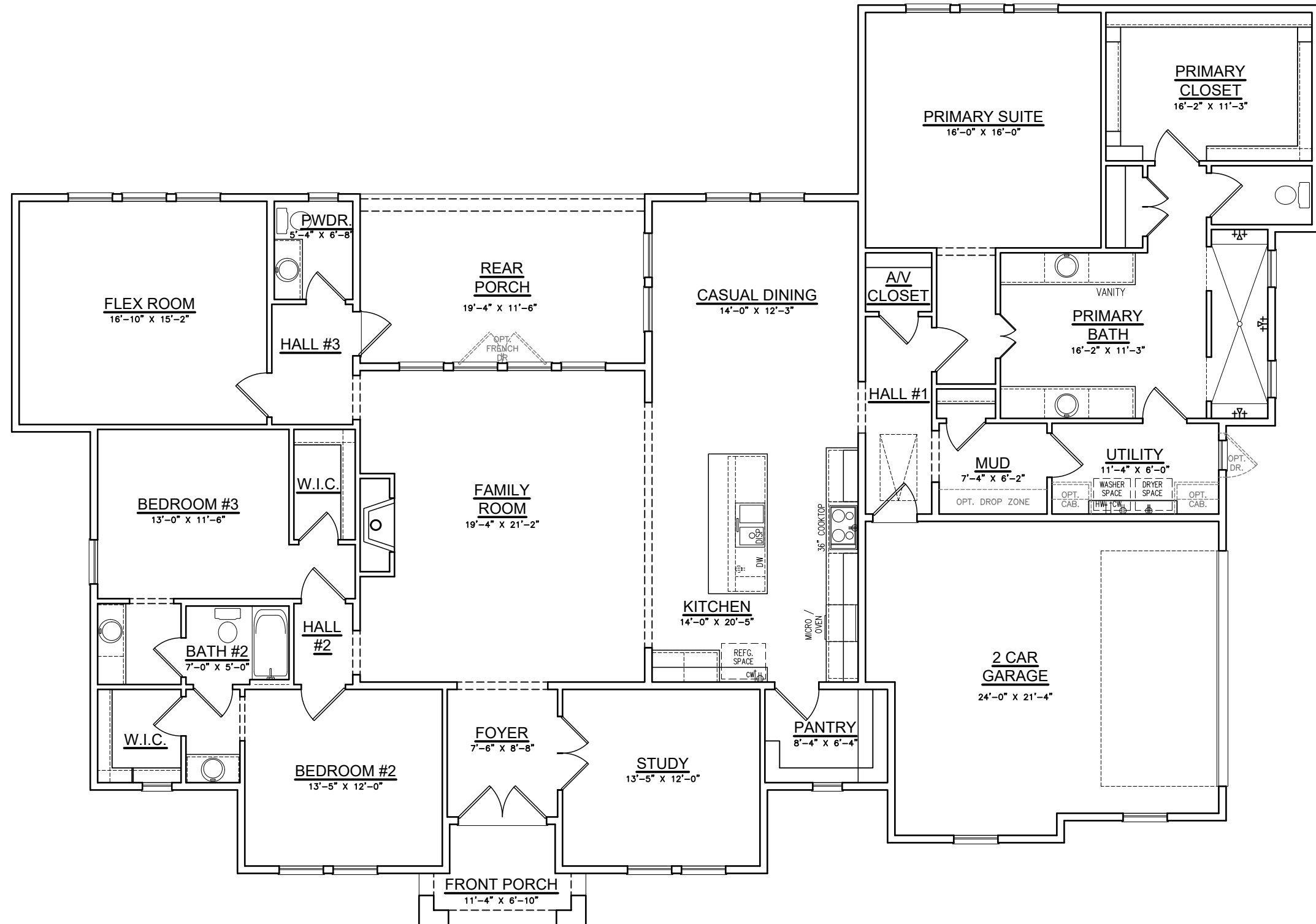
Option #1 Abbott French Revival with Primary Suite Opt. No Primary Bath Tub
