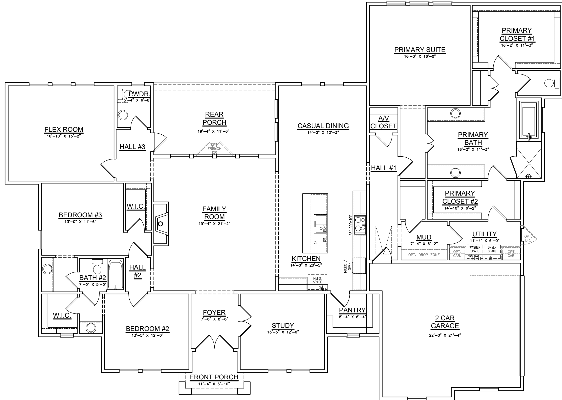
Option #4 Abbott French Revival with Primary Suite Opt. Two Primary Closets
