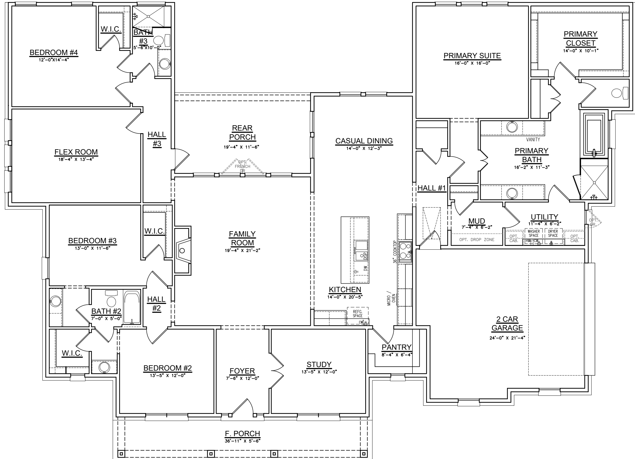
Option #7 Abbott Farmhouse with 4th Bedroom
