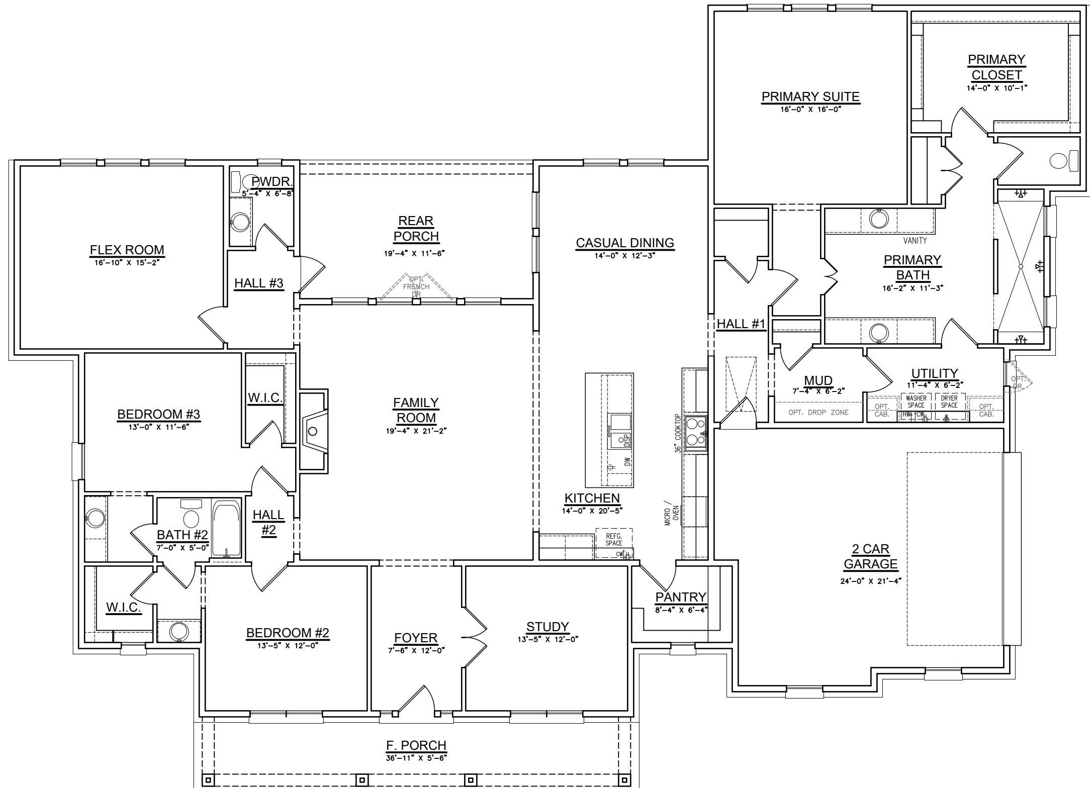
Option #1 Abbott Farmhouse w/ Primary Suite Opt. No Primary Bath Tub
