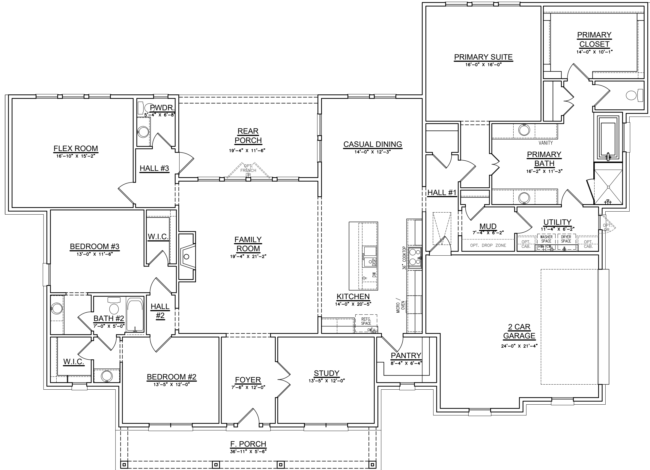
Abbott Farmhouse Base Plan
