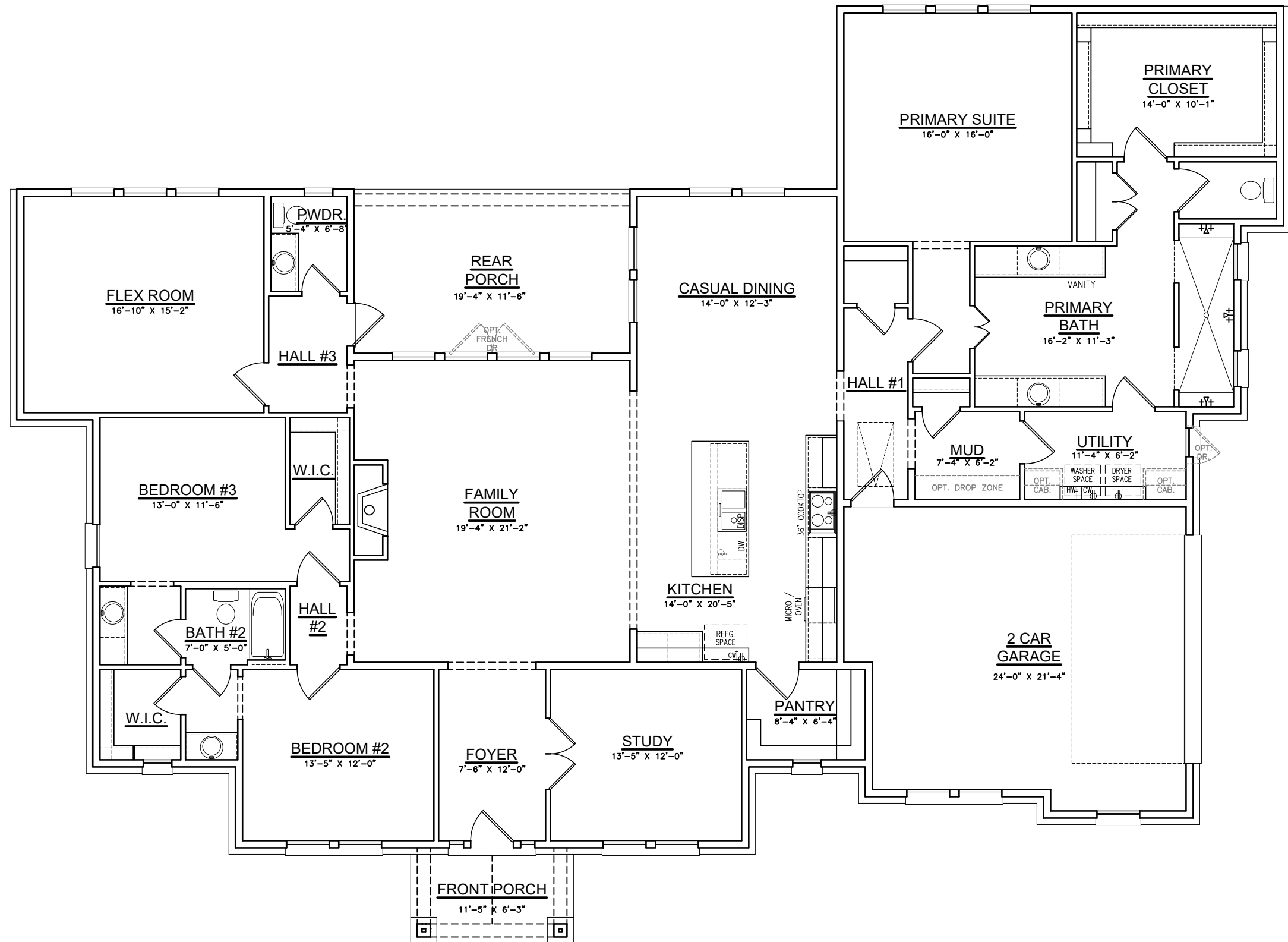
Option #1 Abbott Craftsman w/ Primary Suite Opt. No Primary Bath Tub
