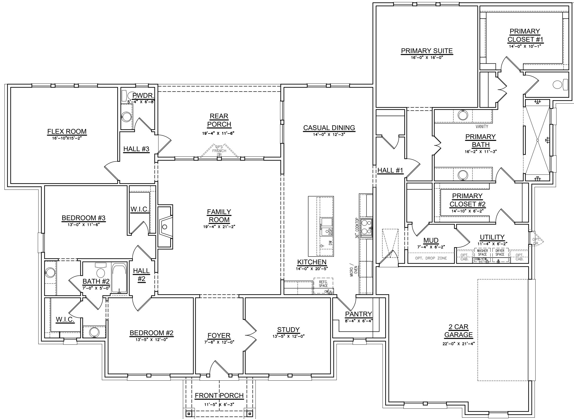
Option #5 Abbott Craftsman w/ Primary Suite Opt. Two Primary Closets w/ No Primary Bath Tub
