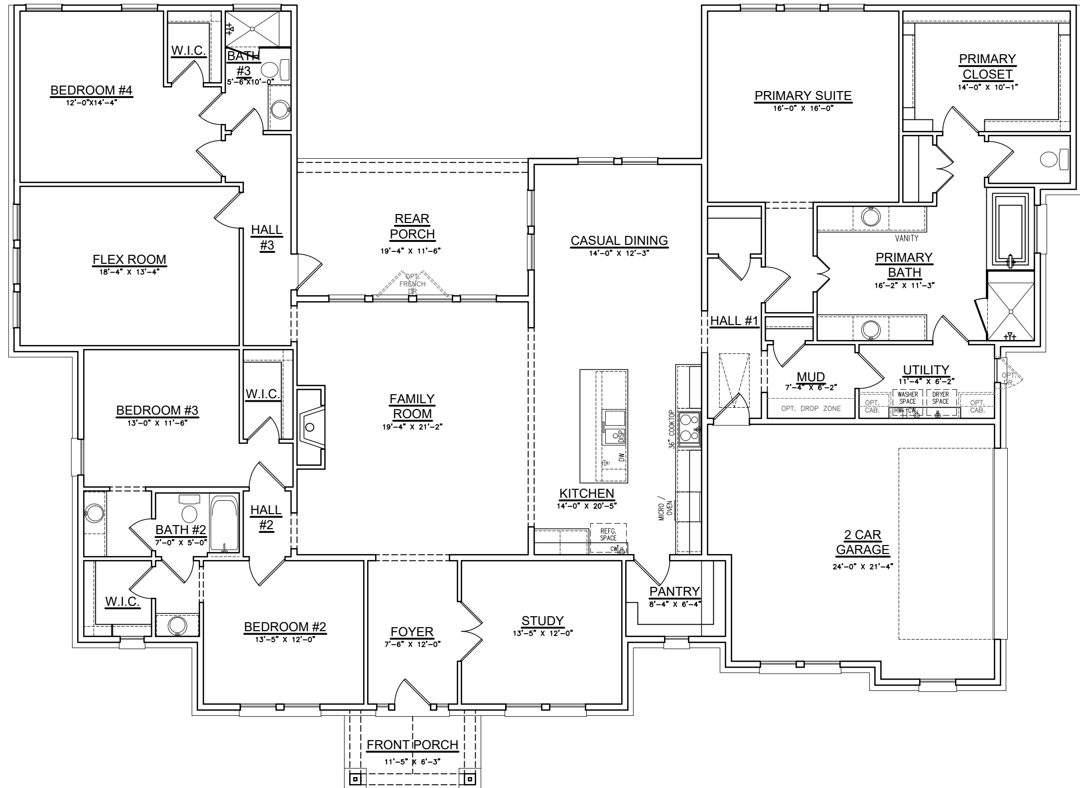
Option #7 Abbott Craftsman with 4th Bedroom
